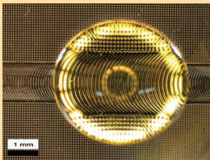
Top view of a 20 \mu l droplet sitting on a ratchet track. The arced rungs constitute the track that is limited by arrays of pillars.
