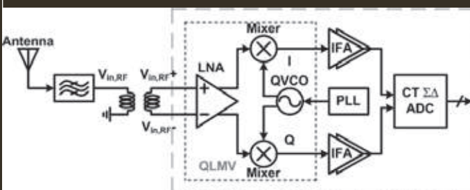
A block diagram of quadrature GPS receiver.
