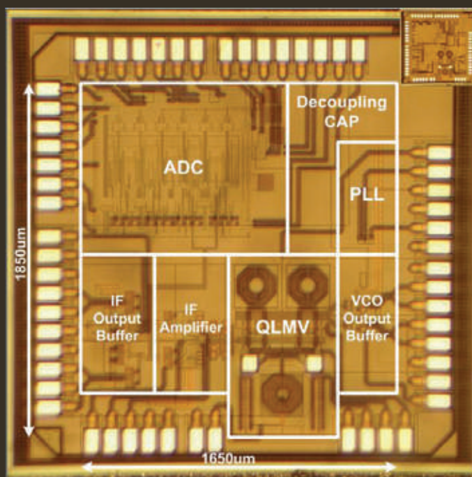
The chip micrograph overlaid on the layout plot for clarity; the die area of the GPS receiver core circuitry (excluding pads) is 1.85mm x 1.65mm.
